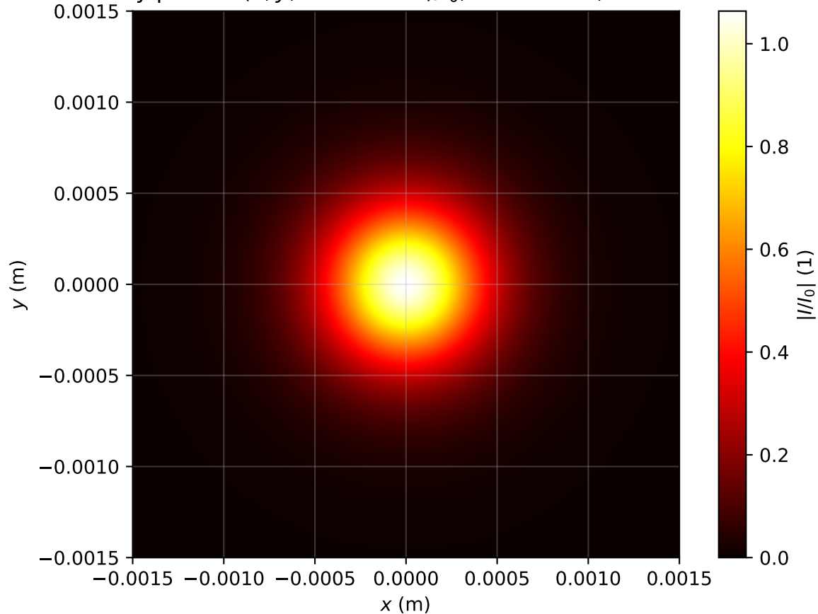
Intensity profile I(x, y, z = 2.149m)/I_0 , P_{in}=0.7P_{cr} , artificial time
